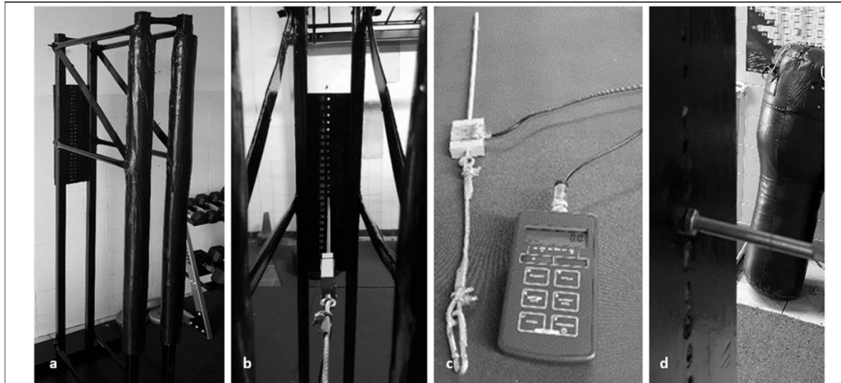
Figure 1. (a) Test frame. b) Threaded bar attachment to anchor board. c) Threaded bar, load cell, display unit, steel cable and carabiner assembly. d) Anchor board height adjustment and threaded bar fixing bolt.
